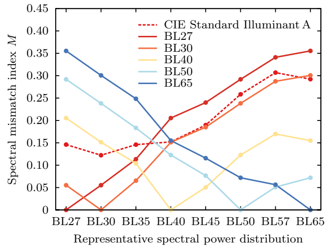
Figure 7. Spectral mismatch index M calculated for Standard Illuminant A and the five candidate representative spectral power distributions.
